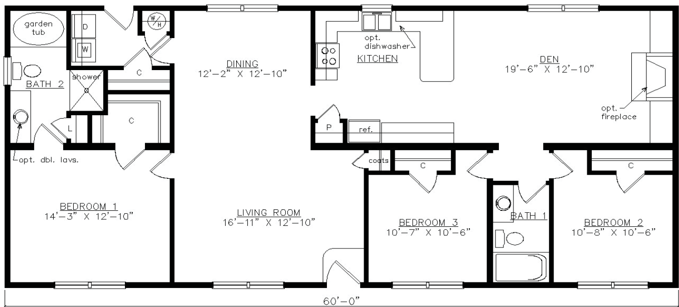
SHOWN WITH OPTIONAL ON-SITE BUILT GABLE PORCH AND FANLITE DOOR 1640 SQ. FT. BEDROOMS: 3 BATHS: 2
