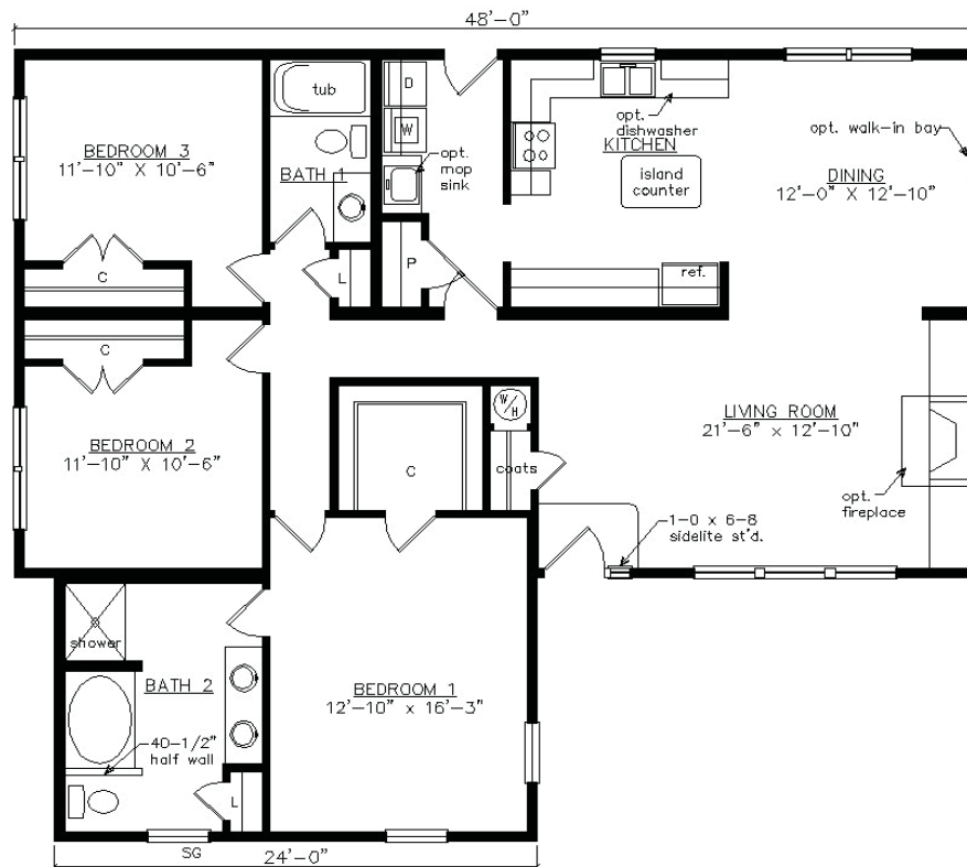
SHOWN WITH OPTIONAL ON-SITE BUILT PORCH, TRIANGLE GABLE VENT, FANLITE DOOR, DOOR SIDELITE AND ACCENT SHAKES 1640 SQ. FT. BEDROOMS: 3 BATHS: 2
