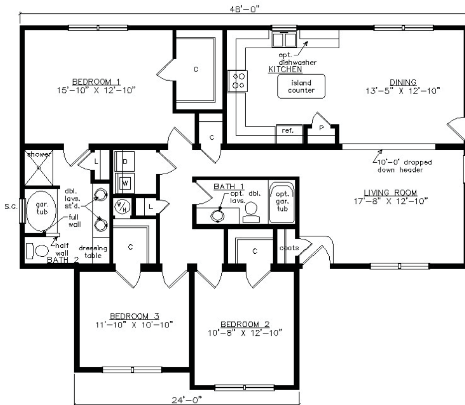
SHOWN WITH OPTIONAL ON-SITE BUILT PORCH AND FANLITE DOOR 1615 SQ. FT. BEDROOMS: 3 BATHS: 2
